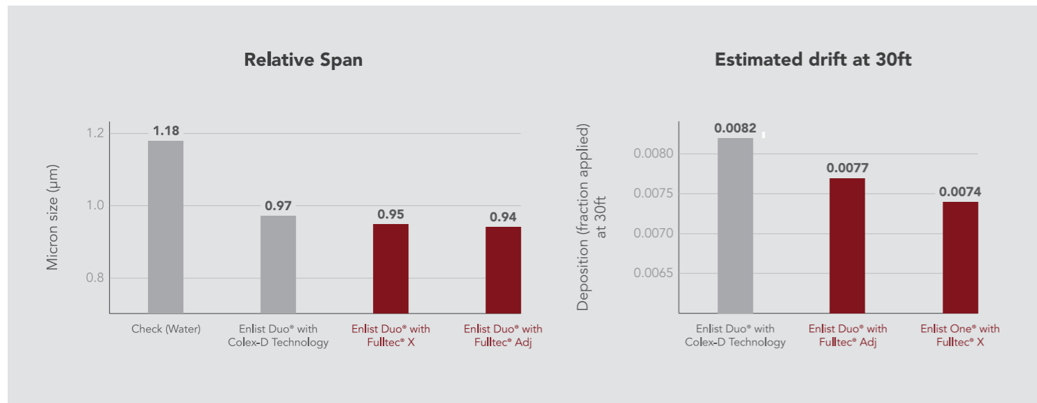
2019 trials - University of Nebraska, West central Research and Extension Center, North Platte, Nebraska. Fulltec X 2.0 oz/acre, Fulltec Adjuvant 2.7 oz/acre. Low speed wind tunnel; AIXR11004 Nozzle at 40 psi.
