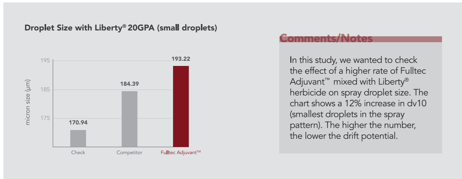
2022 trials - University of Nebraska, West central Research and Extension Center, North Platte, Nebraska. Fulltec Adjuvant 18 oz/100 GAL. Low speed wind tunnel; AIXR11004 Nozzle at 40 psi.
