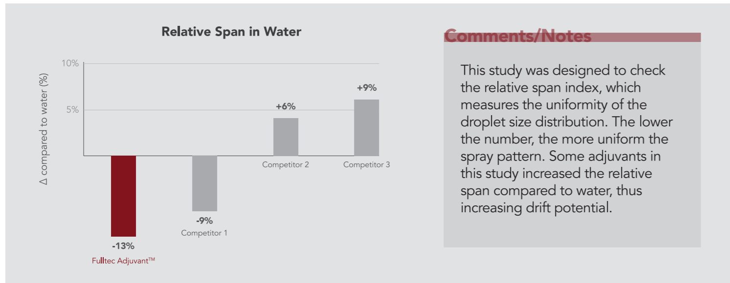
2022 trials - University of Nebraska, West central Research and Extension Center, North Platte, Nebraska. Fulltec Adjuvant 15 oz/100 GAL. Low speed wind tunnel; AIXR11004 Nozzle at 40 psi.
